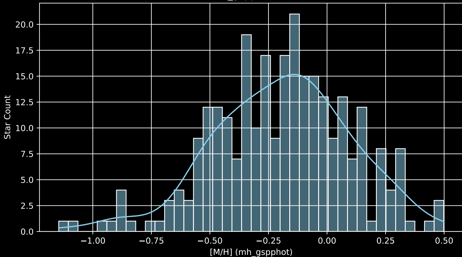
APOGEE DR17 Field: [sgr_tidal6 [M/H] (mh_gspphot) (n= 275)
