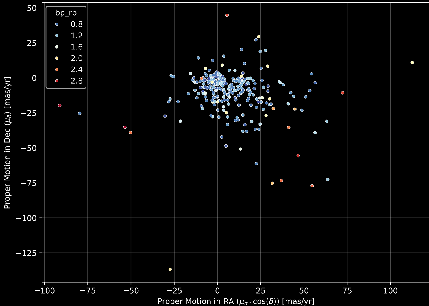
APOGEE DR17 Field: [sgr_tidal6] Proper Motion Diagram (n= 277)
