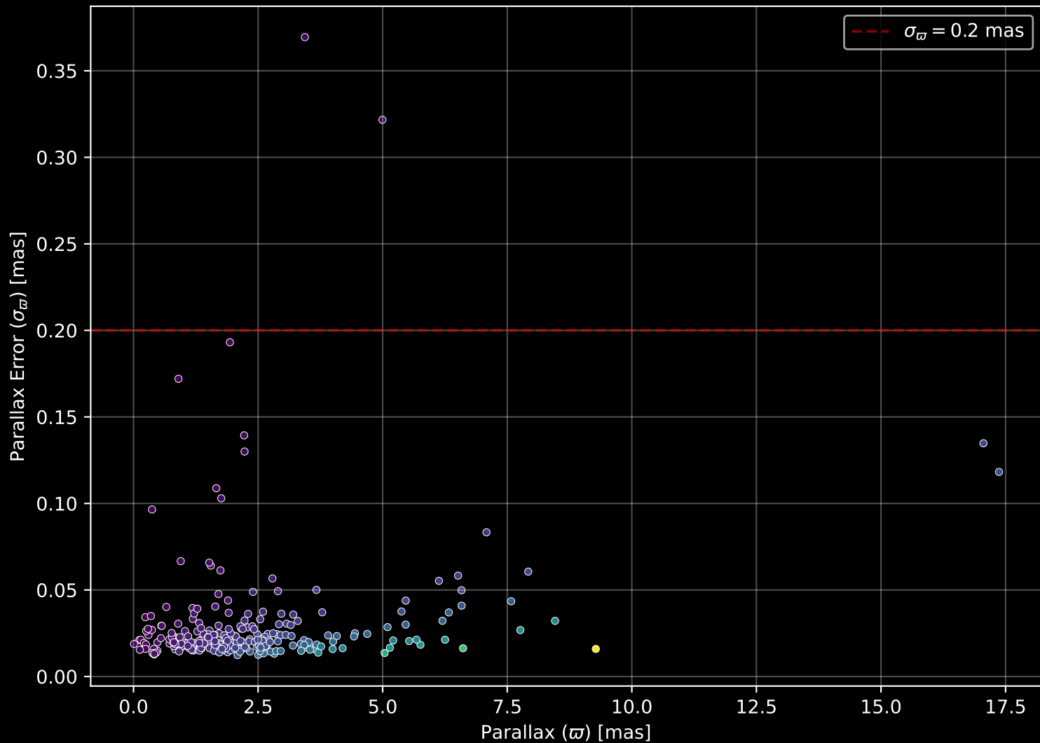
APOGEE DR17 Field: [sgr_tidal6] Parallax Quality (n= 277)
