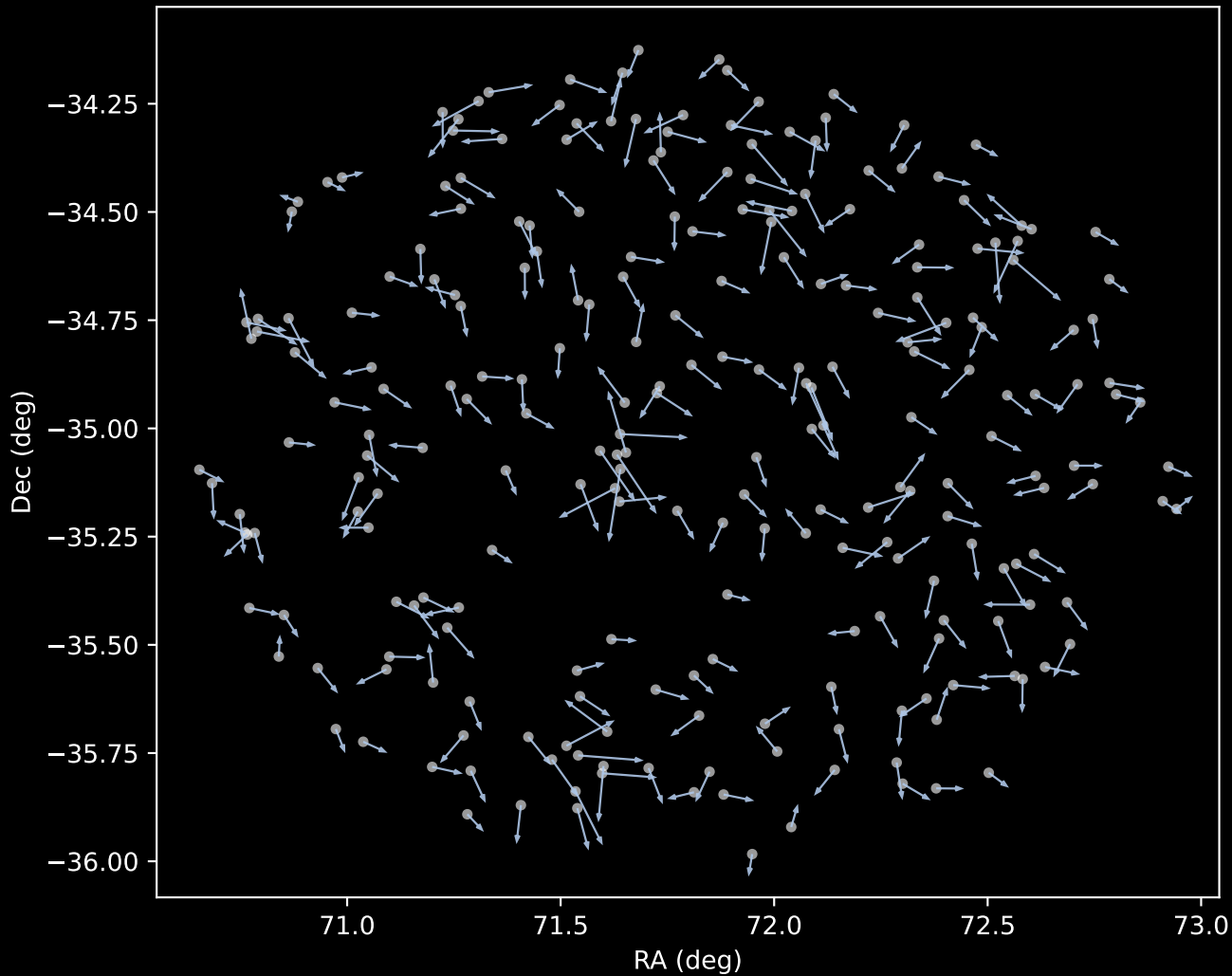
APOGEE DR17 Cluster 1 Proper Motion Vectors (n=244)
