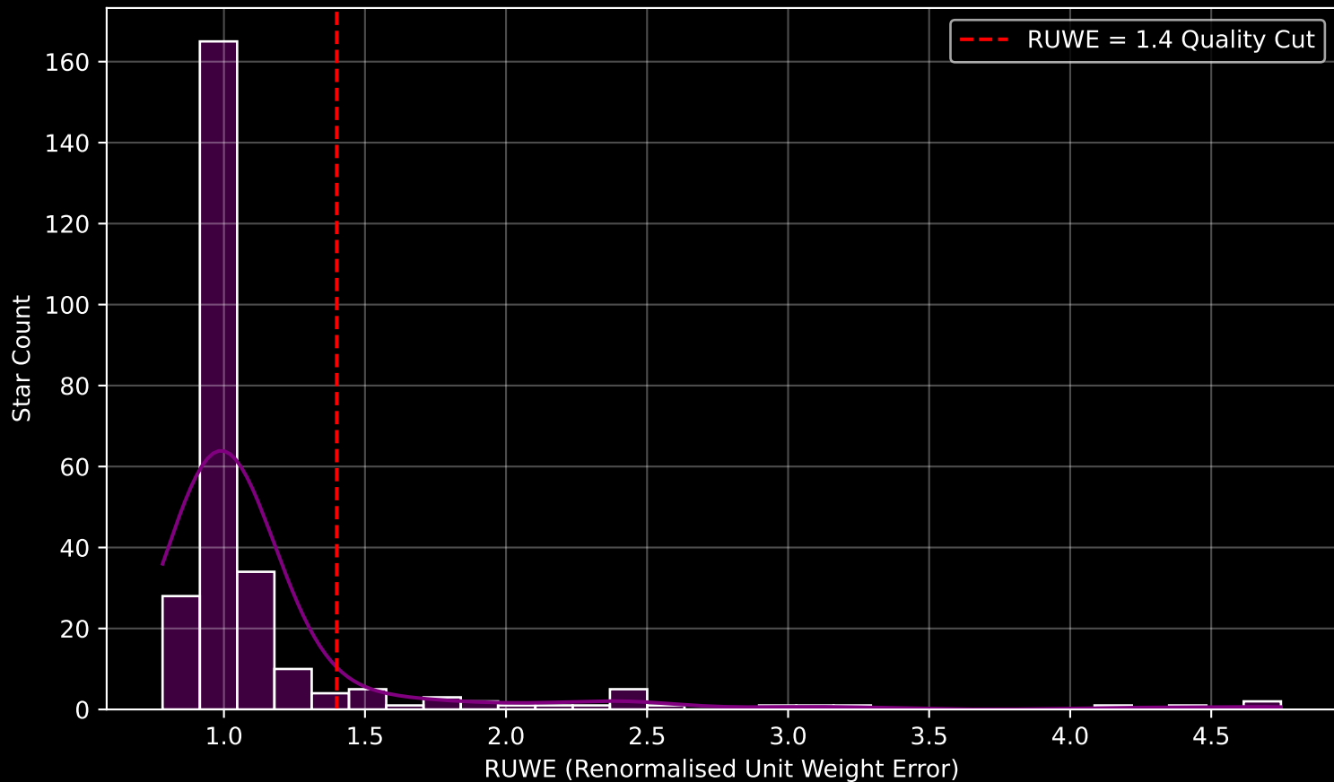
GAPOGEE DR17 Field [sgr_tidal6] RUWE Distribution (n= 268)
