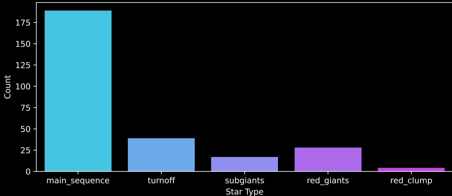
APOGEE DR17 Field: [sgr_tidal6] Count plot of Star Type
